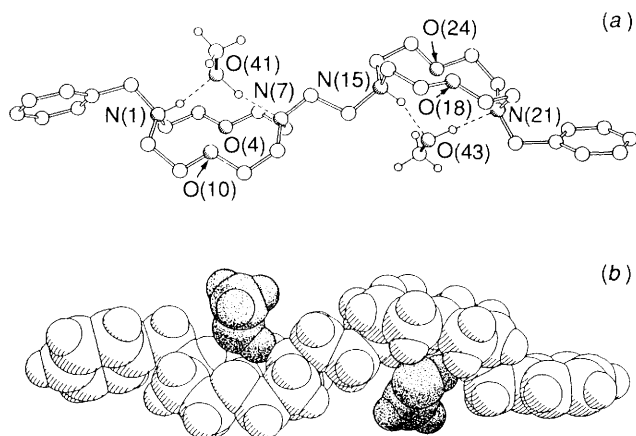
Fig. 4 (a) Framework and (b) space-filling representations of the structure of 5 ·2HPF 6 ·2MeOH in the solid state. In the space-filling representation, the two MeOH molecules are shaded. Transannular [N...N] and [O...O] distances (Å): [N(1)...N(7)], 4.60; [N(15)...N(21)], 4.49; [O(4)...O(10)], 3.02; [O(18)...O(24)], 3.08. Hydrogen-bonding geometries [X...Y] expressed as [X...Y], [H...Y] distances (Å), [X-H...Y] angle (°): [N(1)-H...O(41)], 2.78, 1.83, 169; [O(41)-H...N(7)], 2.91, 1.82, 168; [N(15)-H...O(43)], 2.73, 1.81, 162; [O(43)-H...N(21)], 2.82, 1.82, 178.
