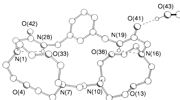
Fig. 2 The structure of 2·MeOH in the crystal. Transannular [N...N] and [O...O] distances (Å): [N(1)...N(7)], 4.61; [N(10)...N(16)], 4.48; [O(4)...O(33)], 3.53; [O(13)...O(38)], 3.60. Hydrogen bonding geometries [X—H...Y] expressed as [X...Y], [H...Y] distances (Å), [X—H...Y] angle (°): [O(43)—H...O(41)], 2.73, 1.78, 171; [N(19)—H...N(16)], 2.71, 2.21, 111; [N(19)—H...O(38)], 3.02, 2.16, 149; [N(28)—H...N(1)], 2.73, 2.24, 111; [N(28)—H...O(33)], 3.16, 2.31, 148.
