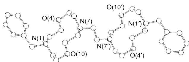
Fig. 3 The structure of 5 in the crystal. The transannular [N...N] and [O...O] distances are 4.30 and 4.32 Å, respectively.
